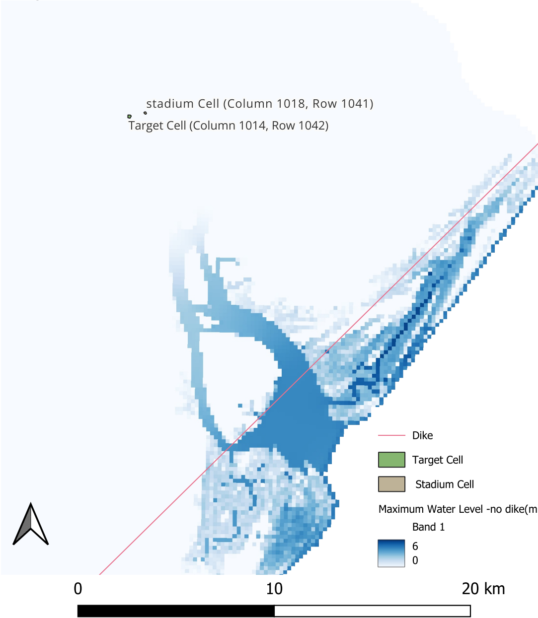
Maximum Water Level — Without Dike Original condition
