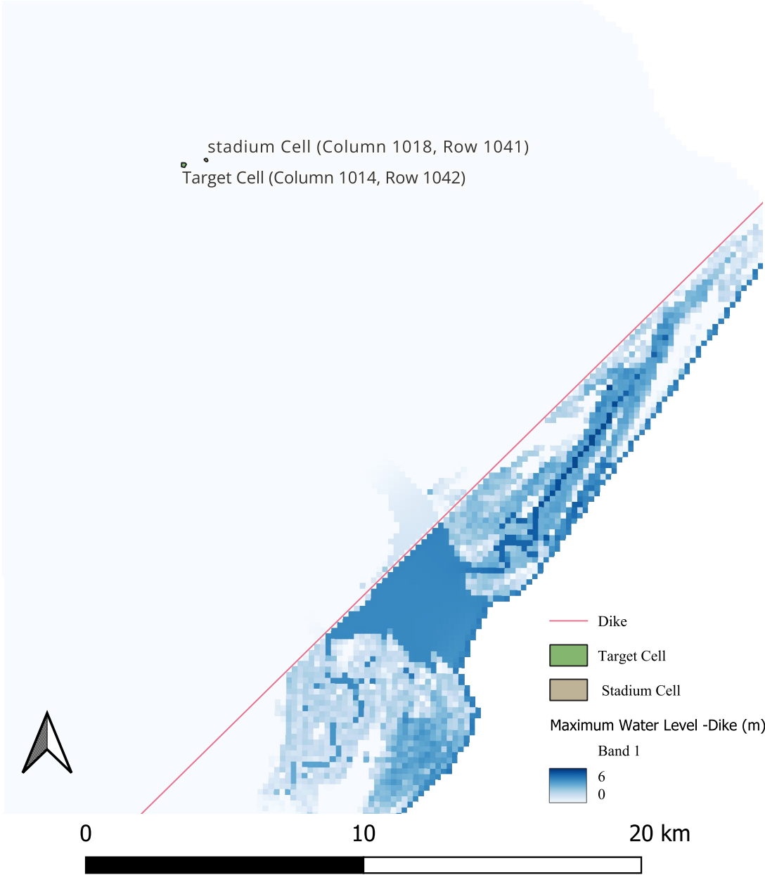
Maximum Water Level — With 4.0m Dike 4.7 m sea-level rise
